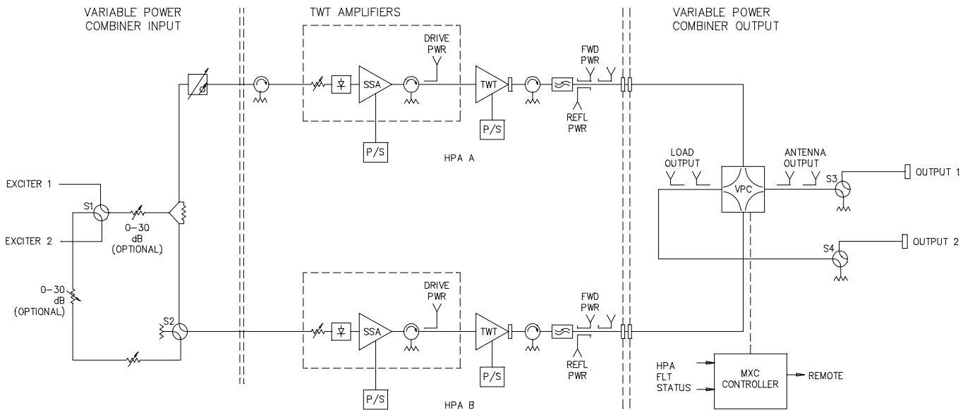
Variable Power Combined/Redundant Configuration
